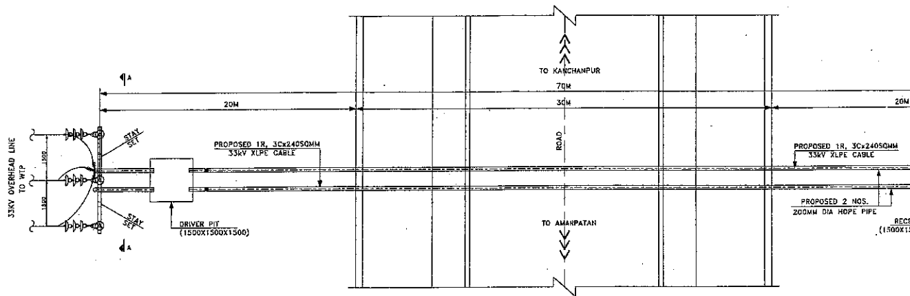
ROAD CROSSING - PLAN
